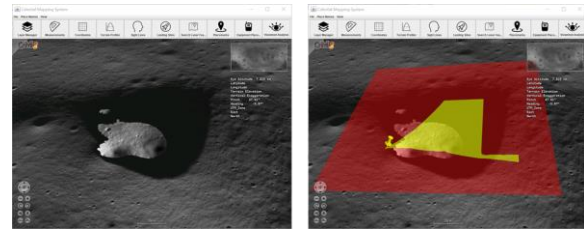
Figure 1: (left) PSR image on top of a high-resolution mosaic of sunlit images of crater, "B01", in Nobile region (right) Viewshed Analysis of the same PSR with observer location shown by yellow pin.
